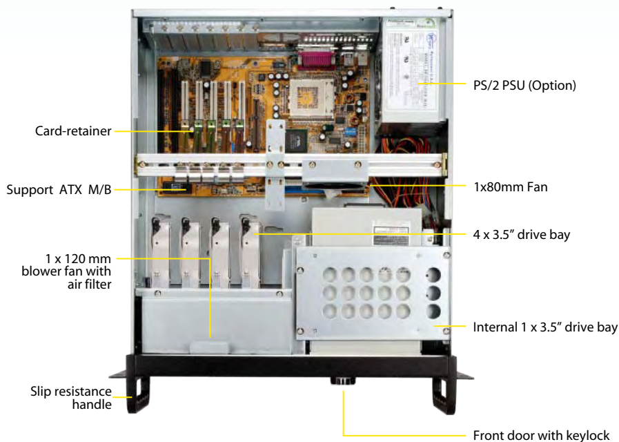
Inside View
