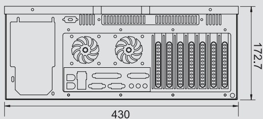
Rear:
