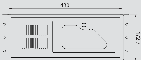
Front 1:
