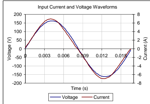
Input AC Current Waveform (ITHD = 6.86%, 50% Load)
