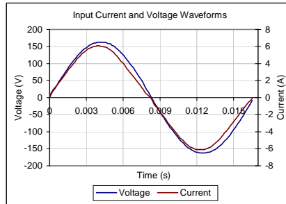
Input AC Current Waveform (ITHD = 5%, 50% Load)
